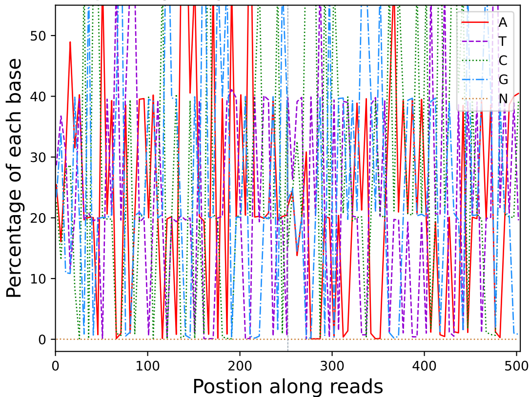
Base percentage along reads (R20206)
